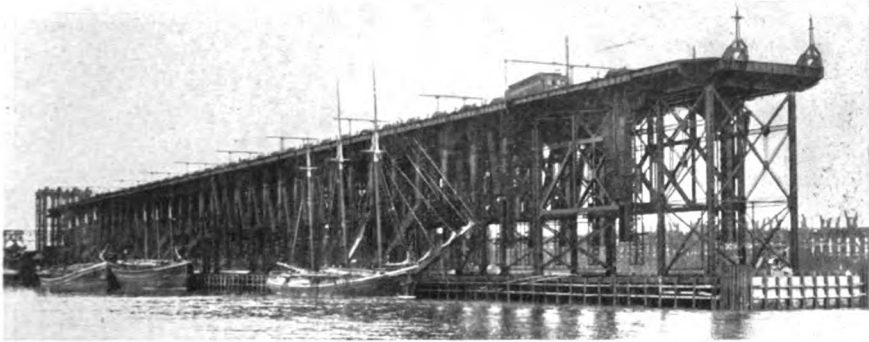
NEW STEEL PIER OF C. & O. RAILWAY AT NEWPORT NEWS, VA.
